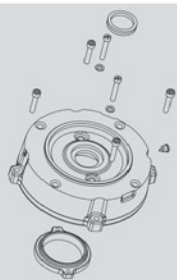
C-Din Flange Kit
