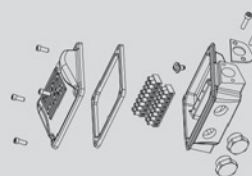
Auxiliar Terminal Box Kit
