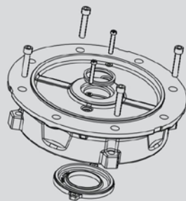
FF Flange Kit
