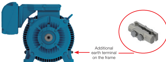
Figure 6 - Additional earth terminal position on the frame.
