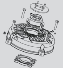
Drive endshield Kit - W3Seal
