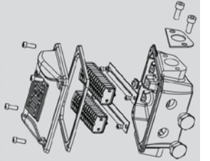
Auxiliar Terminal Box Kit
